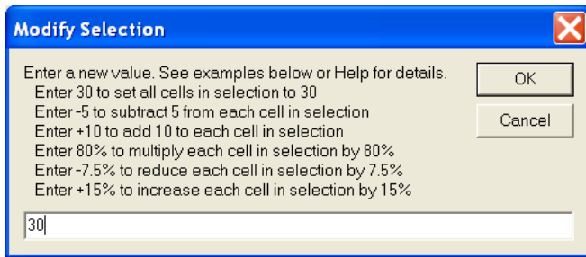
Figure 19 – Modify Command
