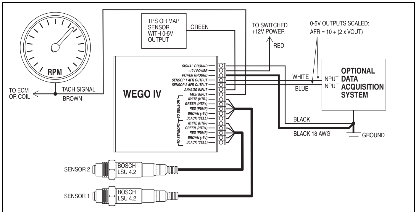
Figure 1 - WEGO IV Dual Channel Hookup
